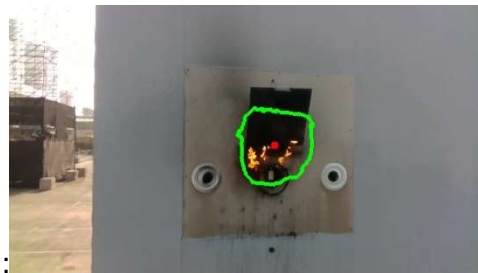
Figure 2.6: Fire detection
